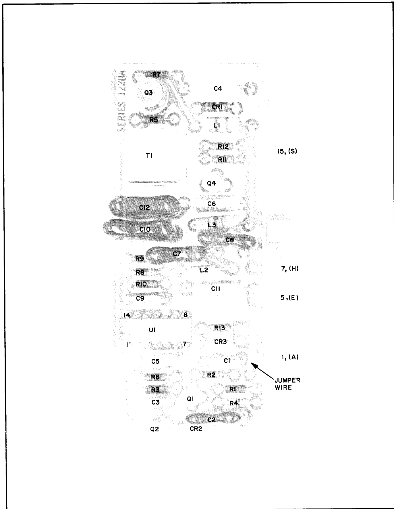
Part of Figure 8-6. A7 1.0 MHz to 100.0 kHz Divider Board
