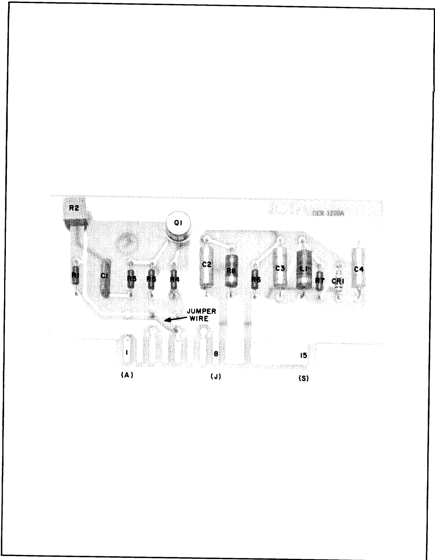
Part of Figure 8-4. A5 Input Amplifier
