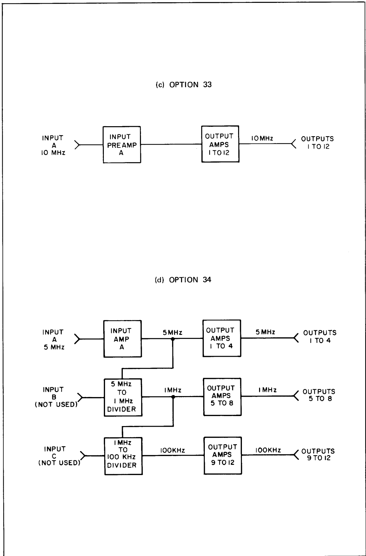
Figure 4-1. 5087A Block Diagram (Continued)
