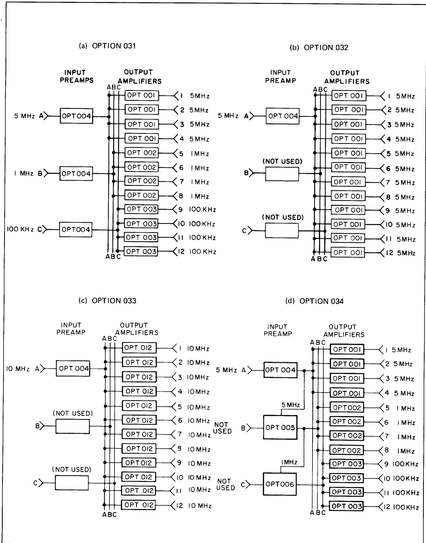
Figure 1-1. Available Configurations
