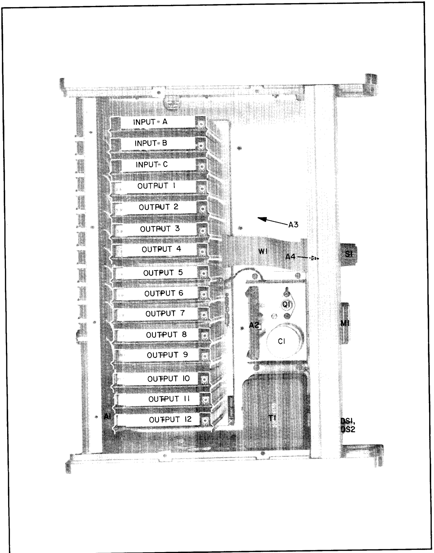
Part of Figure 8-2. Model 5087A Top View Shield Off
