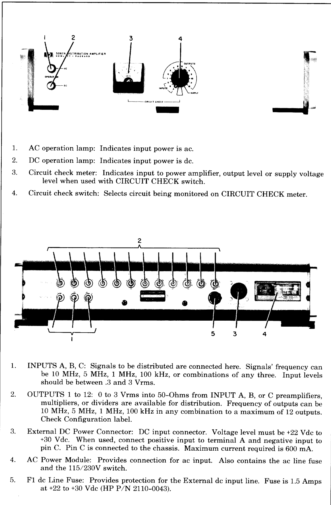
Figure 3-2. Front and Rear Panel Controls, Indicators, and Connectors
